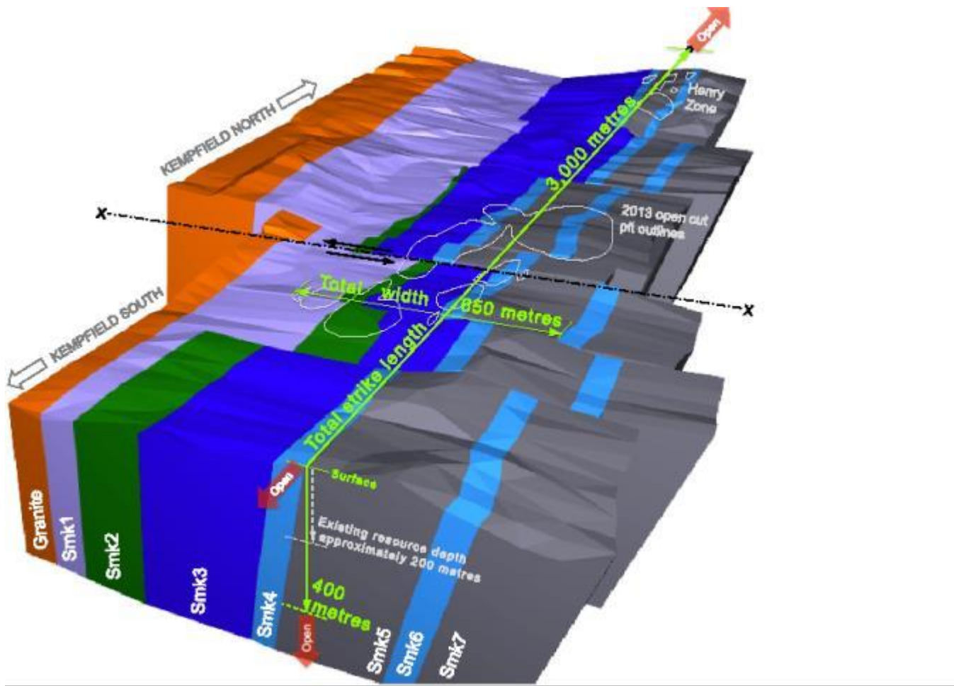
Figure 3 – Open Pit Design
